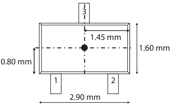
21.2 SOT Package
