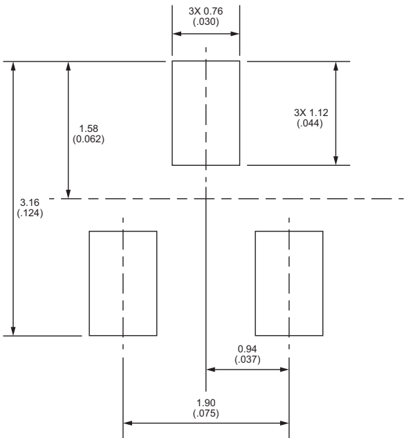
26.1 SOT -23-3 Solder Pad Layout
