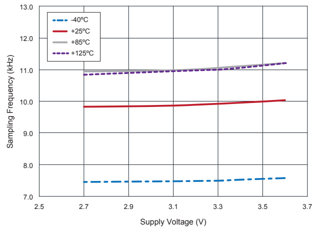
16.28 RR121-1B93-312 Sampling Frequency vs. Supply Voltage vs. Temperature
