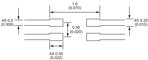
26.3 Leaded LGA-4 Solder Pad Layout
