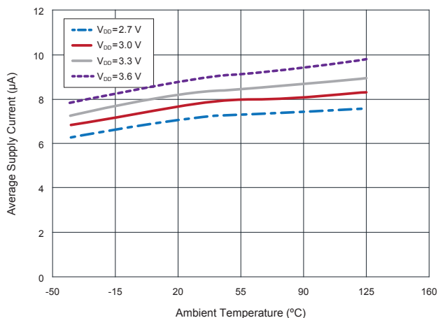
16.26 RR121-1E73-311 and RR121-3C73-311 Average Supply Current vs. Temperature vs. Supply Voltage
